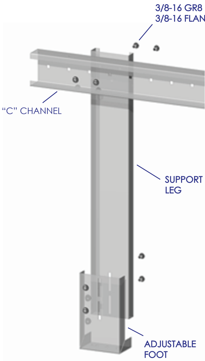
SUPPORT LEG
